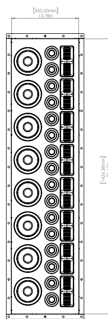
BAFFLE ASSEMBLY INSTALLED
